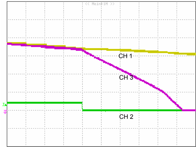
Figure 2: Input voltage turn-off threshold (2mS/div): CH1: Vin (VRTN_AF reference to -48V_AF, 10V/div). CH2: lin (-48V_AF, 2A/div). CH3: VRTN_OUT reference to -48V_OUT (10V/div).
